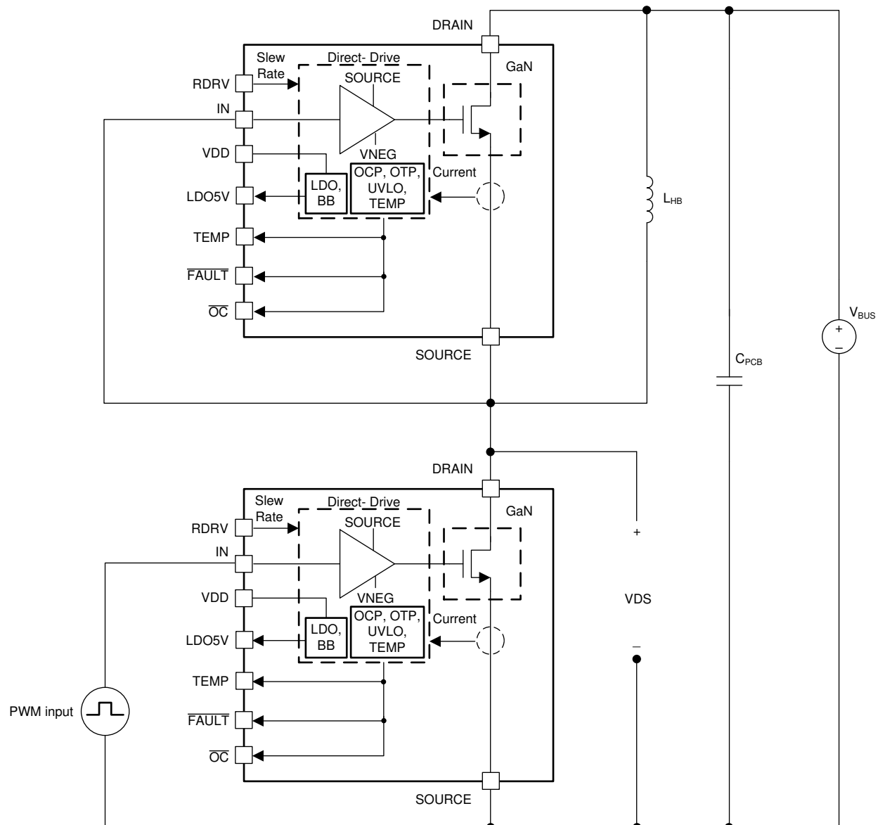
8-1. Circuit Used to Determine Switching Parameters
