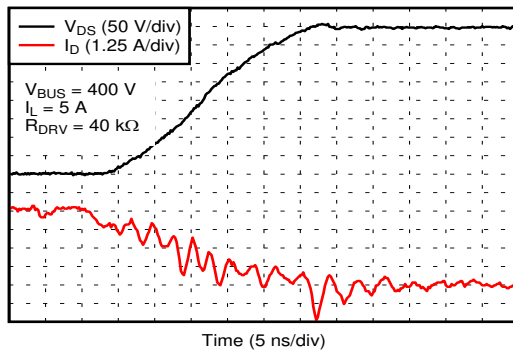
10-4. Turn-Off Waveform in Application Example
